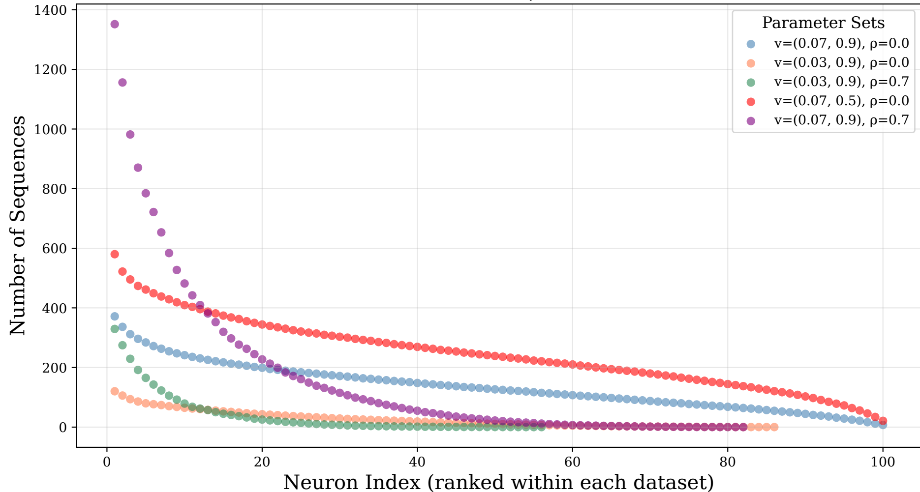
Average Neuron Participation Across Sequences of 50 Subsamples \sigma=(0.02, 0.4) \mid R=100
